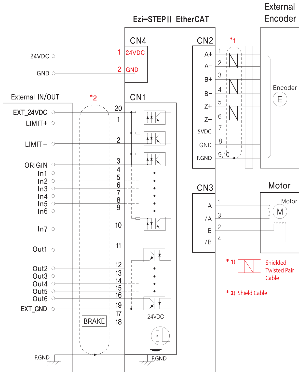
Figure 2.3: External Wiring Diagram of Ezi-STEP II EtherCAT
