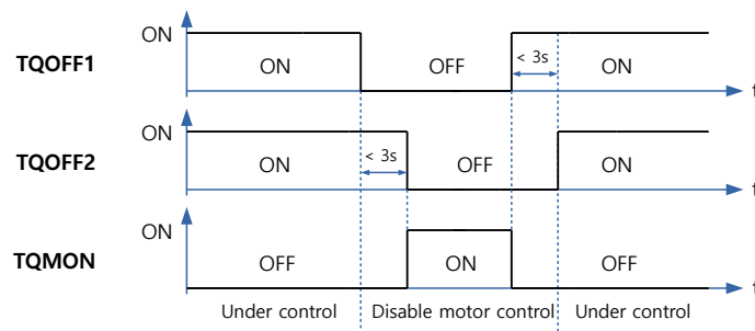
Figure 4.19: TQOFF Input (Normal Operation 1)
