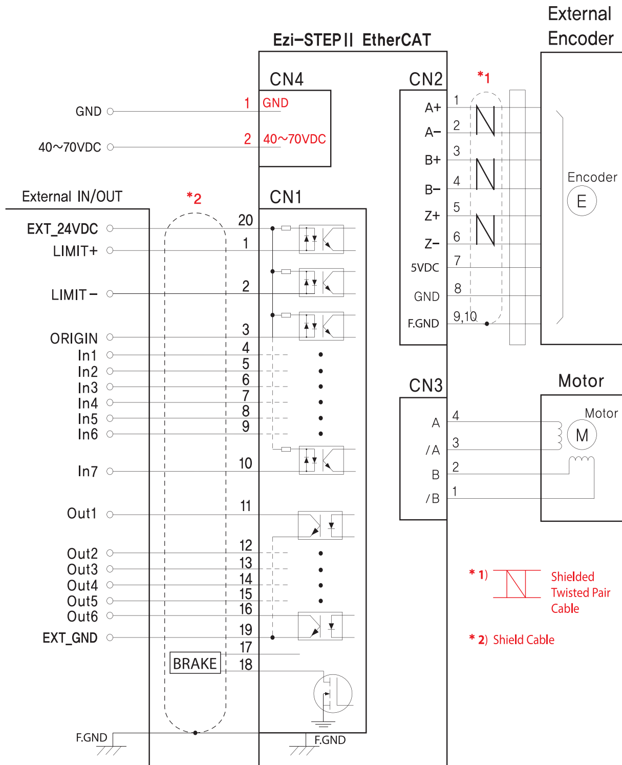
Figure 2.4: External Wiring Diagram of Ezi-STEP II EtherCAT 86
