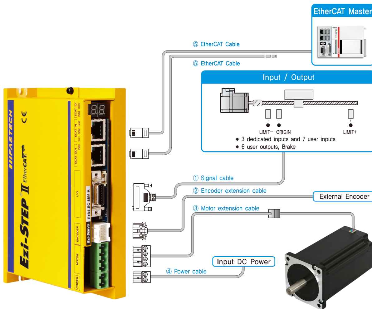
Figure 2.2: System Configuration Diagram of Ezi-STEP II EtherCAT 86
