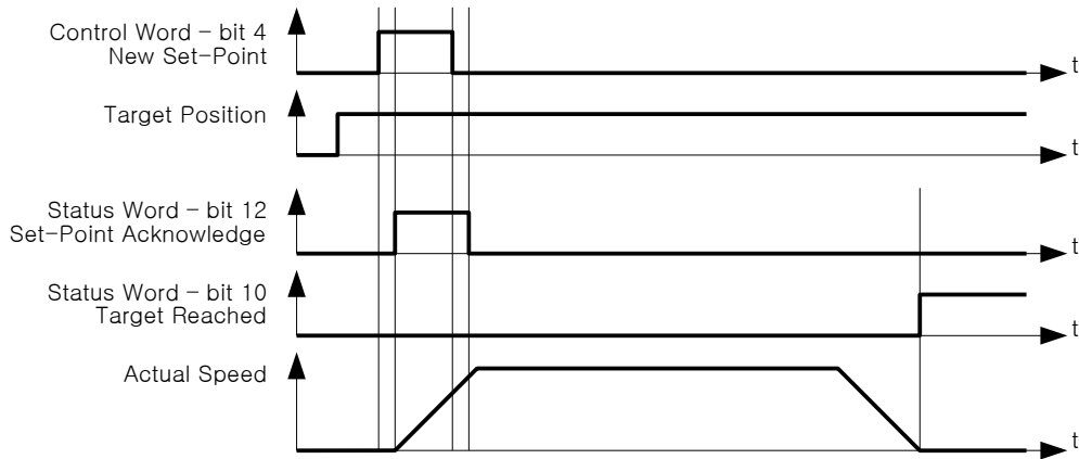
Figure 4.4: New Set-Point
