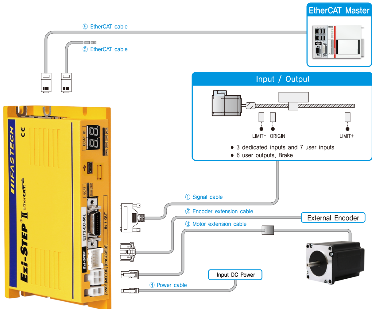
Figure 2.1: System Configuration Diagram of Ezi-STEP II EtherCAT
