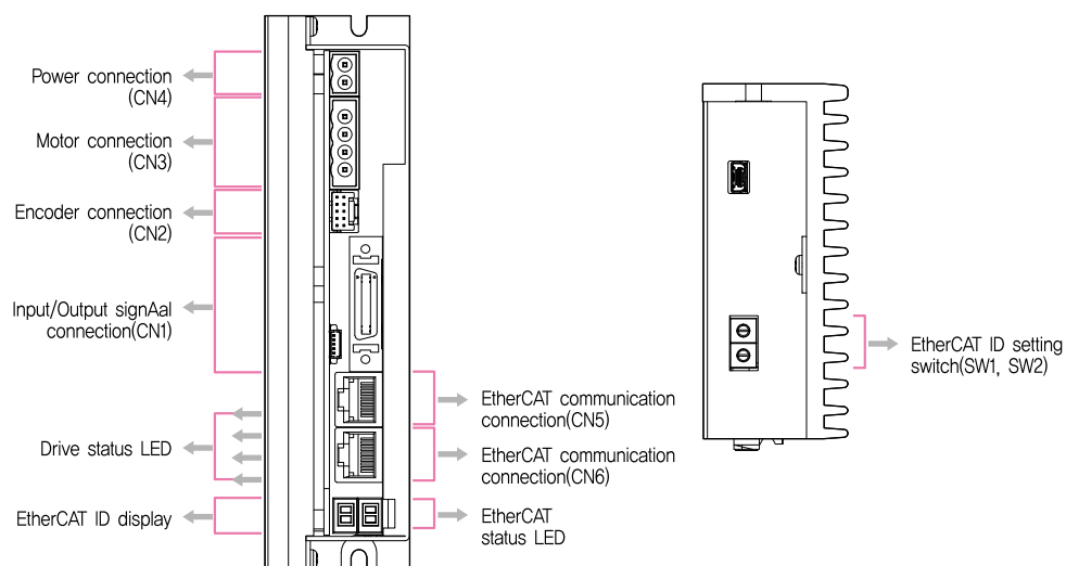
Figure 2.6: Appearance of Ezi-STEP II EtherCAT 86
