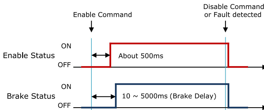
Figure 4.17: Brake Signal
