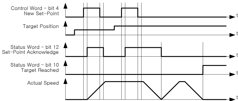
Figure 4.5: Next Set-Point
