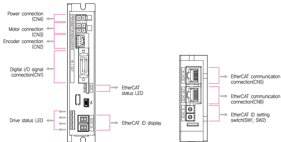
Figure 2.5: Appearance of Ezi-STEP II EtherCAT
