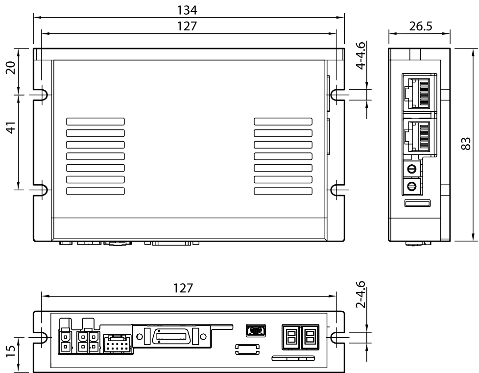
Figure 1.2: Dimensions of Ezi-STEP II EtherCAT
