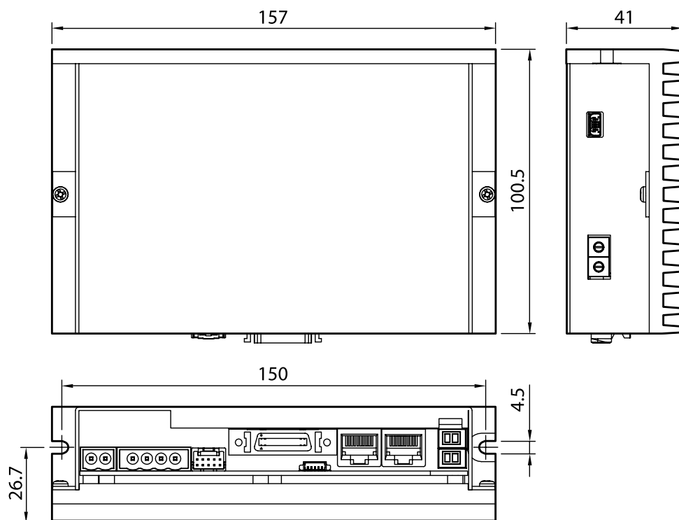
Figure 1.3: Dimensions of Ezi-STEPII EtherCAT 86
