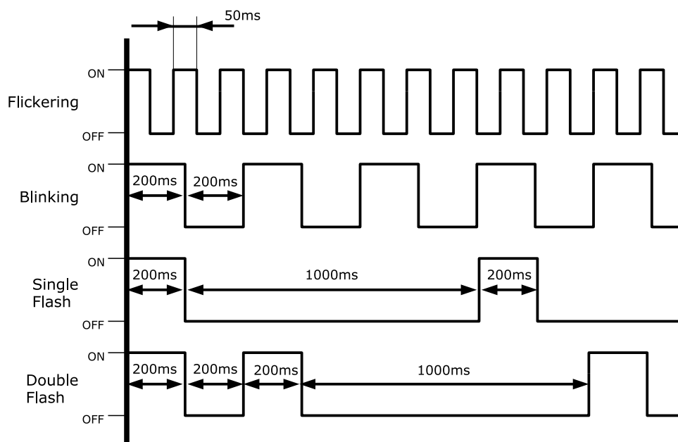
Figure 2.5: EtherCAT LED
