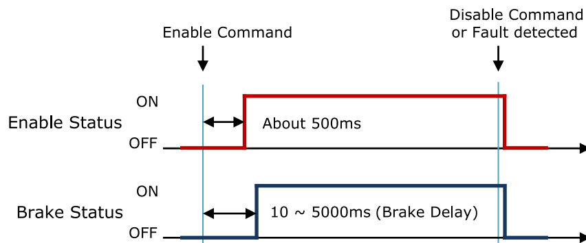
Figure 4.17: Brake Signal
