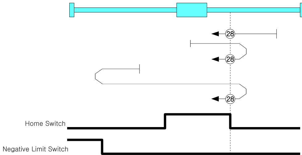
Figure 4.12: Homing Method 28
