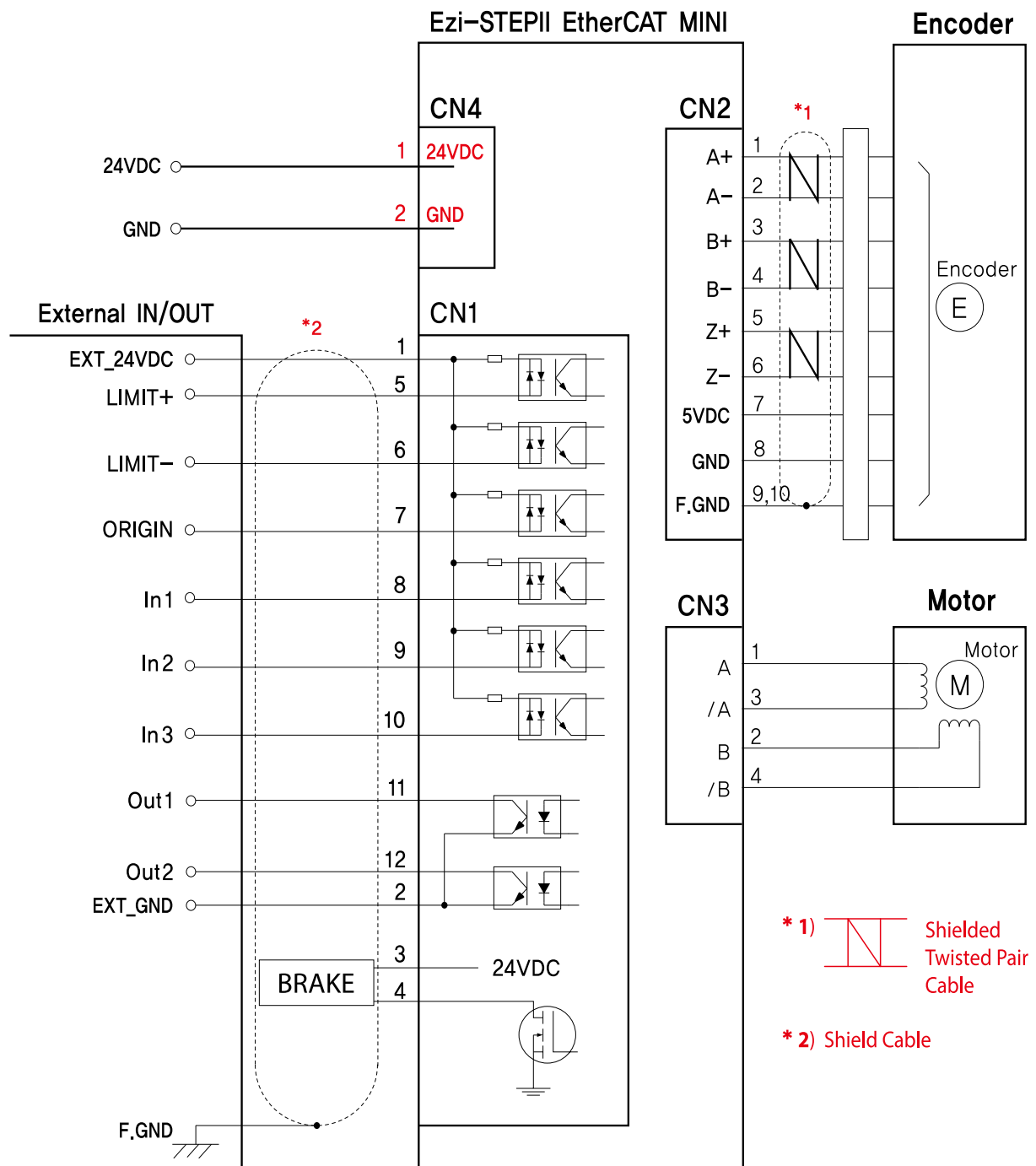
Figure 2.2: External Wiring Diagram of Ezi-STEPII EtherCAT MINI
