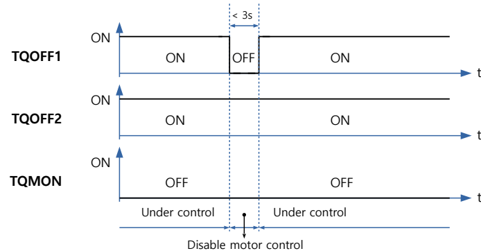
Figure 4.20: TQOFF Input (Normal Operation 2)
