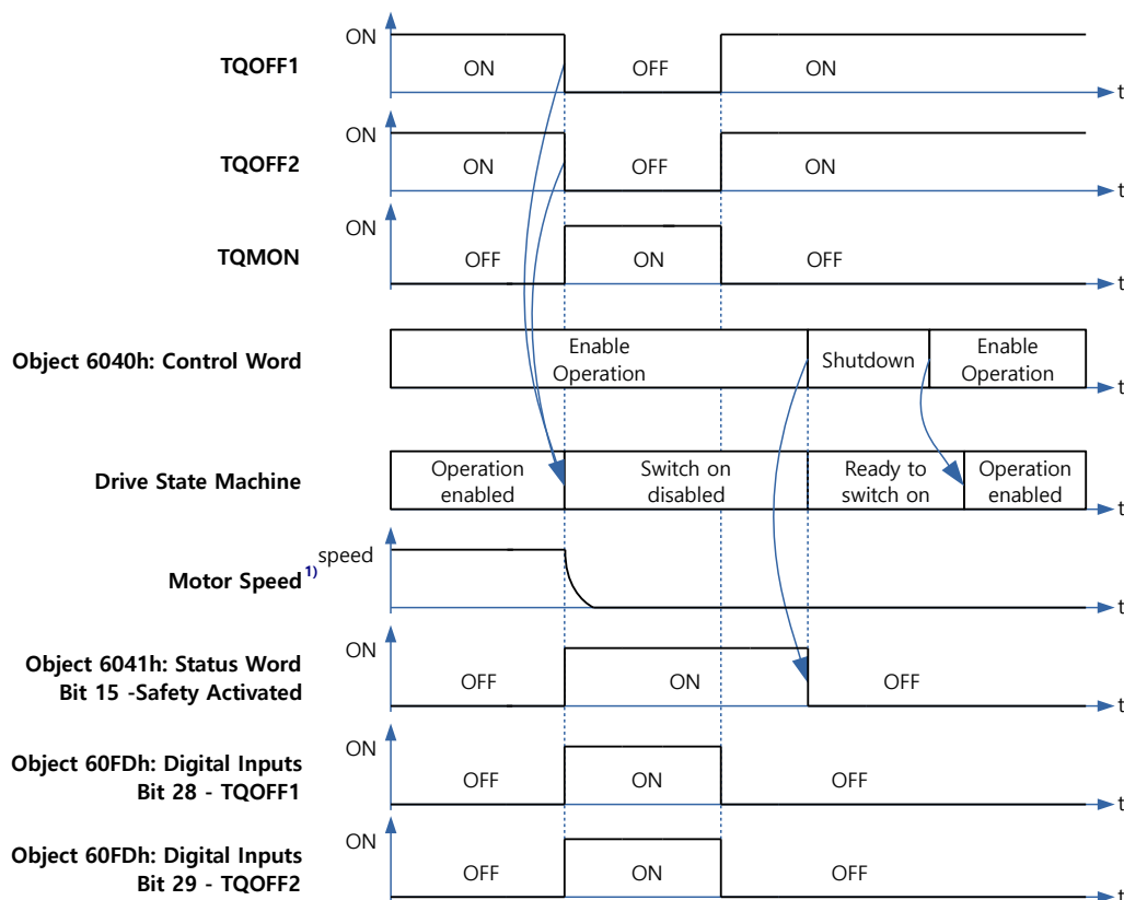
Figure 4.18: Safety Function Timing Chart
