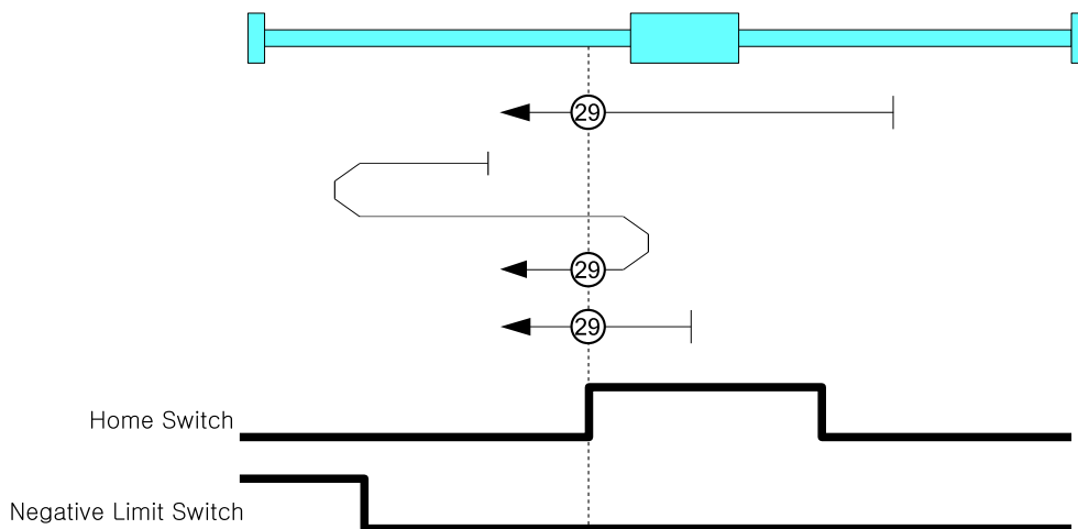
Figure 4.13: Homing Method 29
