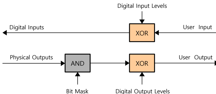
Figure 4.16: Digital I/O Level
