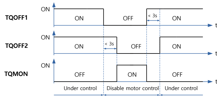
Figure 4.19: TQOFF Input (Normal Operation 1)
