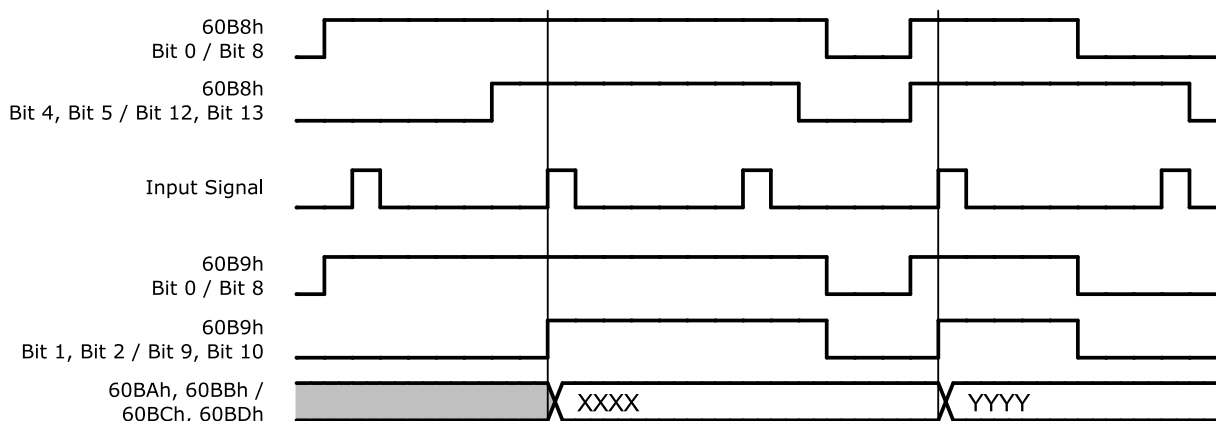
Figure 4.14: Touch Probe Operation (Bit 1 / Bit 9 = 0)
