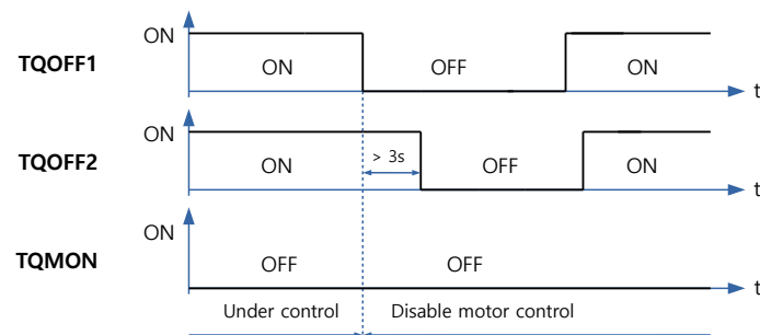
Figure 4.21: TQOFF Input (Fault Operation)
